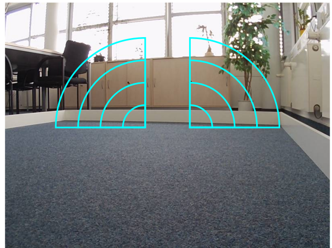
Fig. 11. An exemplary view of the front camera.
