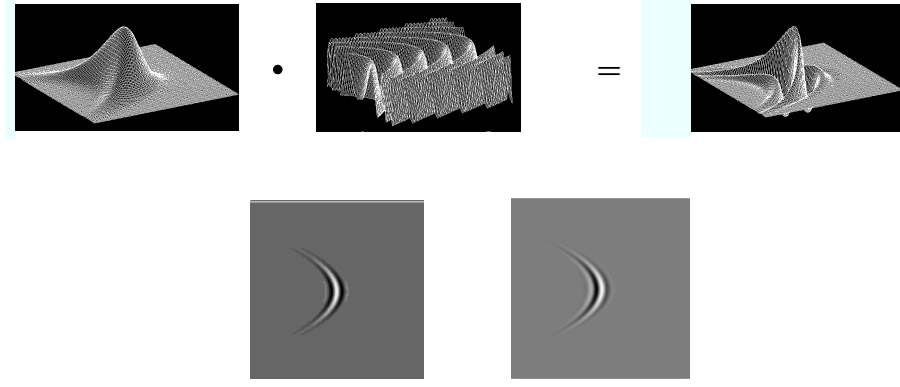
Figure 3: Top: Real part of a banana wavelet is the product of a curved Gaussian G^{\bar{b}}(x, y) and a curved wave function F^{\bar{b}}(x, y) . Bottom: Real and imaginary part of the same banana wavelet depicted as grey level picture, with white encoding high values.
